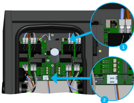
Figure 8: Location of the Ethernet port (1) and SIM card holder (2)
