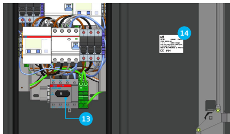
Figure 2: main switch (13), identification label (14)
