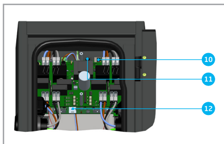
Figure 1 Controllerboard
