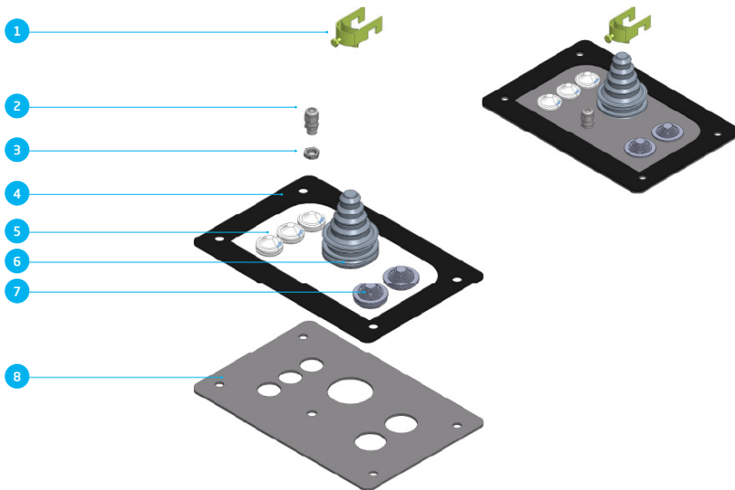
Figure 5: Bottom assembly overview
